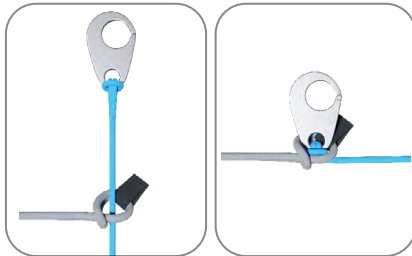
Diagram 1. Speed-bar connection by means of the Brummel hook. The blue line is from the harness, and the gray from the riser.
