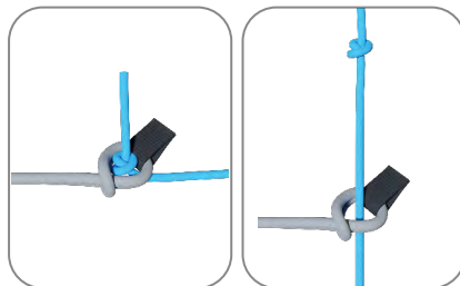
Diagram 2. Speed-bar connection by means of kite loop (without Brummel hook). The blue line is from the harness, and the gray from the riser.
